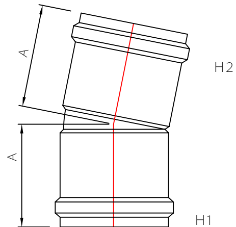
FABRICATED FITTING(F)
