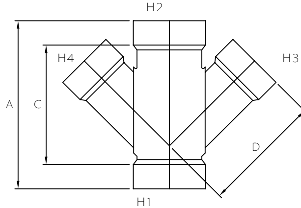
FABRICATED FITTING (F)
