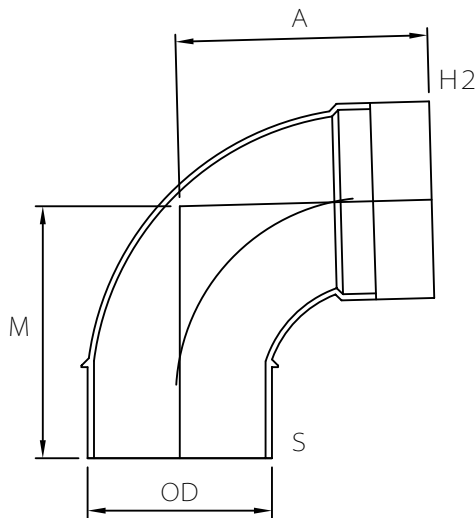
INJECTION MOLDED FITTING (M)
