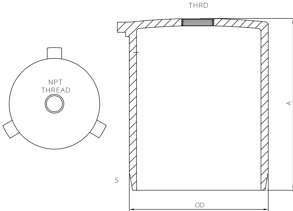
FABRICATED FITTING (F)
