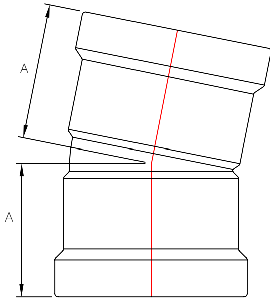
INJECTION MOLDED FITTING (M)
